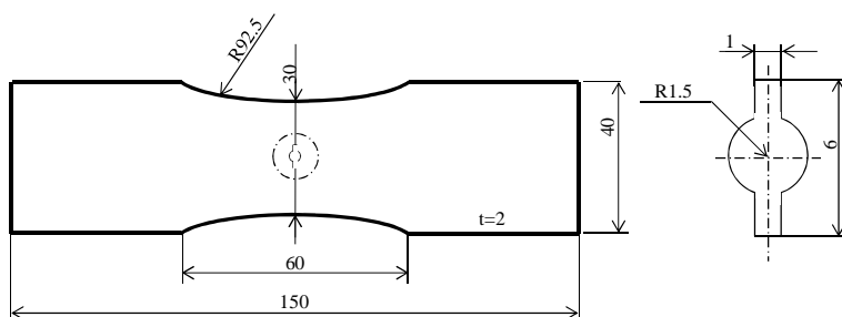
Fig. 2 Shape of specimen for fatigue crack propagation rate test.
