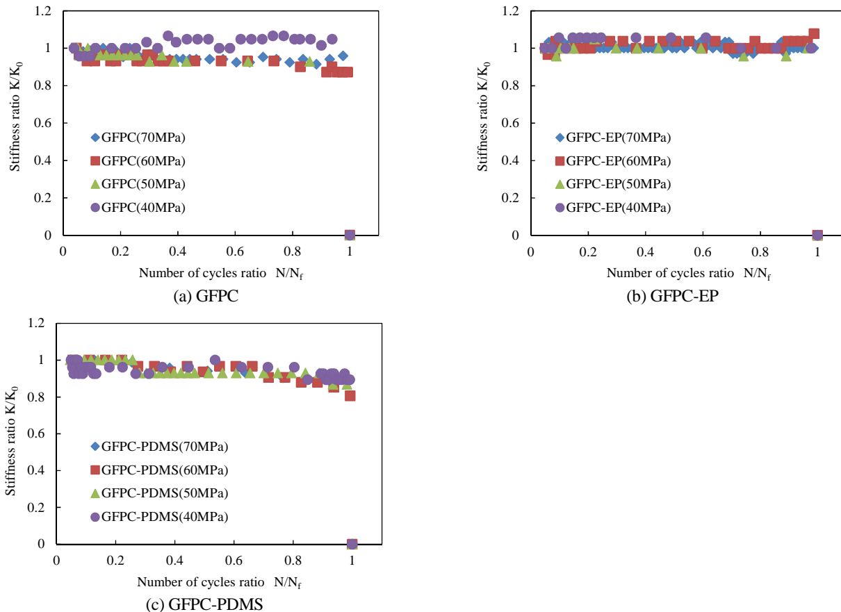
Fig. 10 Stiffness ratios of fatigue test at stress rate R=0 and frequency f=3\text{Hz} . The results for \sigma_{max}=70, 60, 50 and 40\text{MPa} are plotted with the diamond-shaped (blue), square (red), triangle (green) and circle (purple), respectively. In GFPC and GFPC-PDMS, stiffness ratios decrease with increasing the number of fatigue loads. However, in GFPC-EP, it does not decrease.
