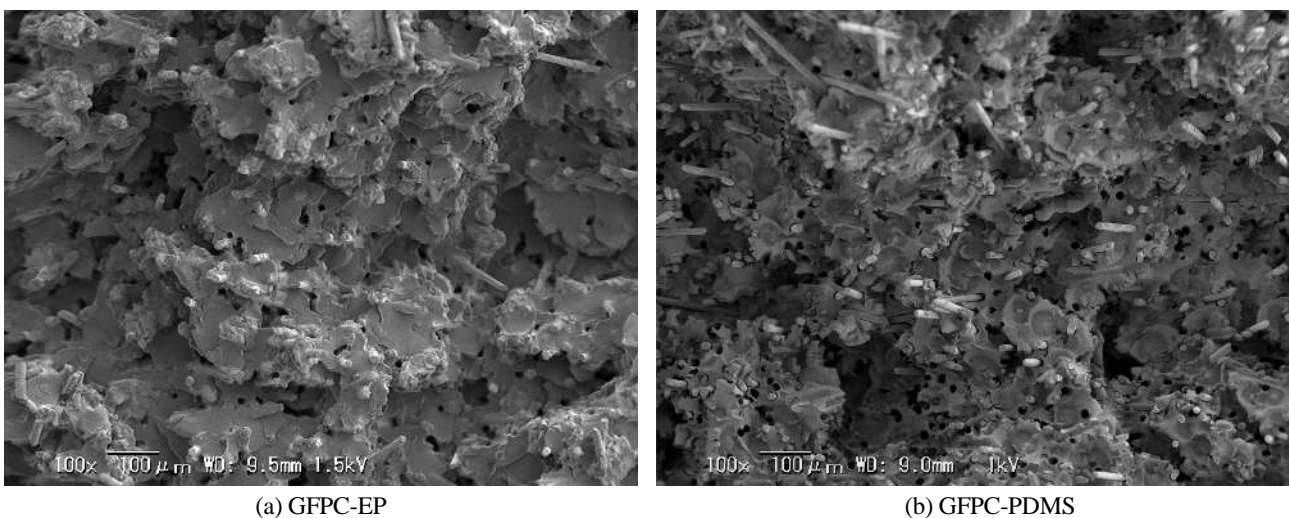
Fig. 11 SEM wide area observation images of the fracture surfaces of fatigue test. ( \sigma_{max}=70\text{MPa} ) In GFPC-EP, the cracks initiate at several fiber ends. In GFPC-PDMS, cracks initiate at almost all fiber ends.
