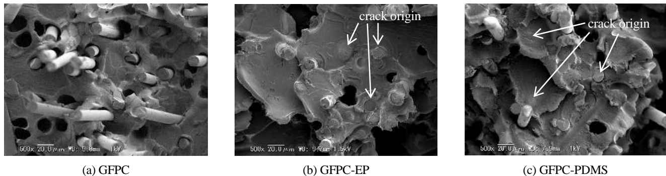
Fig. 6 SEM micrographs of fracture surfaces of fatigue test. ( \sigma_{\max} = 70\text{MPa} ). In GFPC, GF exposed from PC is observed all the area of the fracture surface. Space is formed between PC at the bottom of exposed GF. In PC-EP and PC-PDMS, there is no exposed GF and most GFs are fractured. The interface is not debonded in most cases under high stress amplitude.
