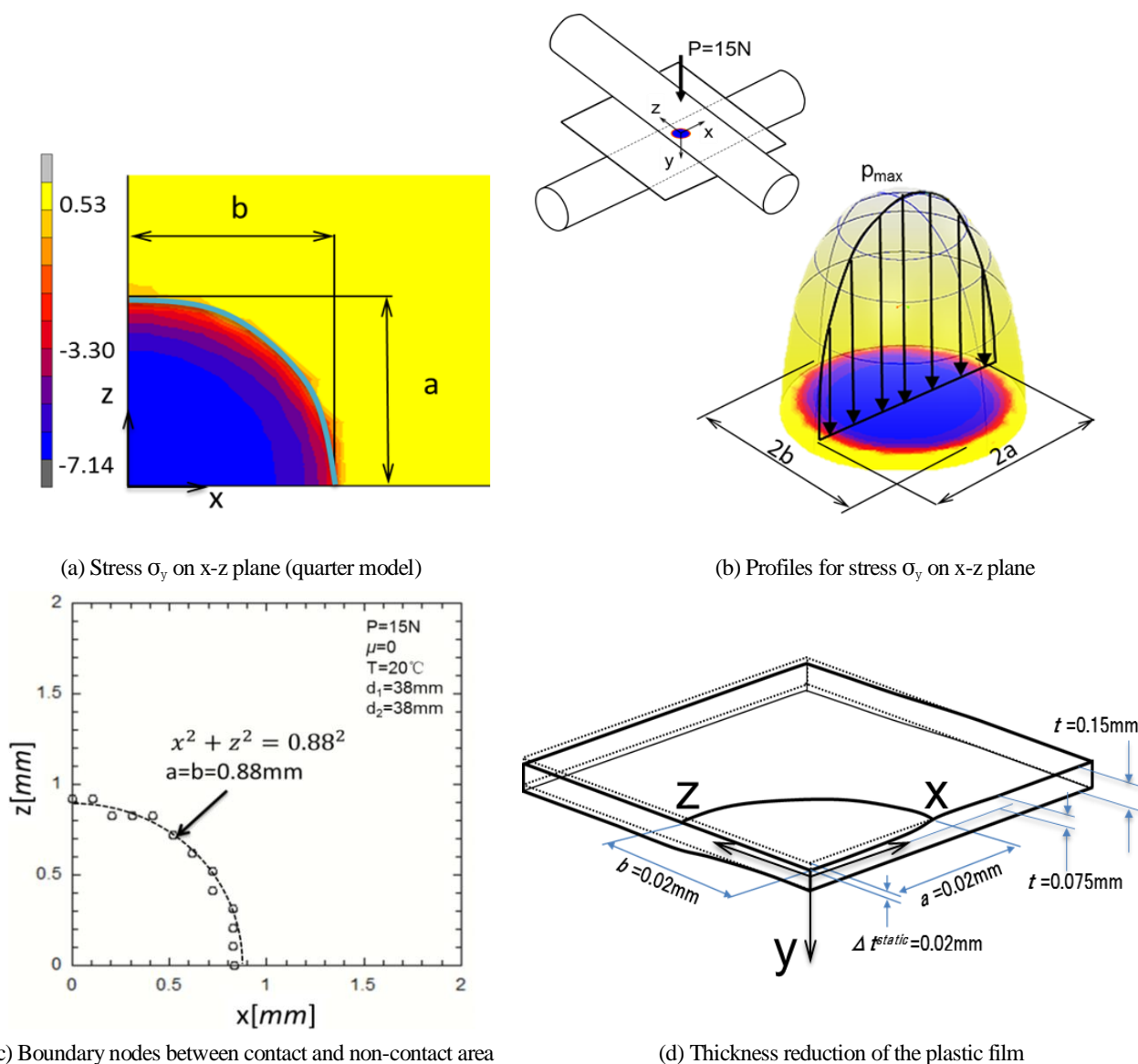
Fig. 8 The stress and deformation of the film when P=15\text{N} , \mu=0 , T=20^\circ\text{C} and d_1=d_2=38\text{mm} . (a) Stress \sigma_y at the contact area on the x-z plane. (b) The maximum stress at x-z plane is p_{max}=7.14[\text{MPa}] appears on the center of plastic film. (c) Contact area with dimensions a=b=0.88 (dotted line). (d) The maximum thickness reduction appears at the center of the plastic film ( \Delta t/2=0.01\text{mm} ).
