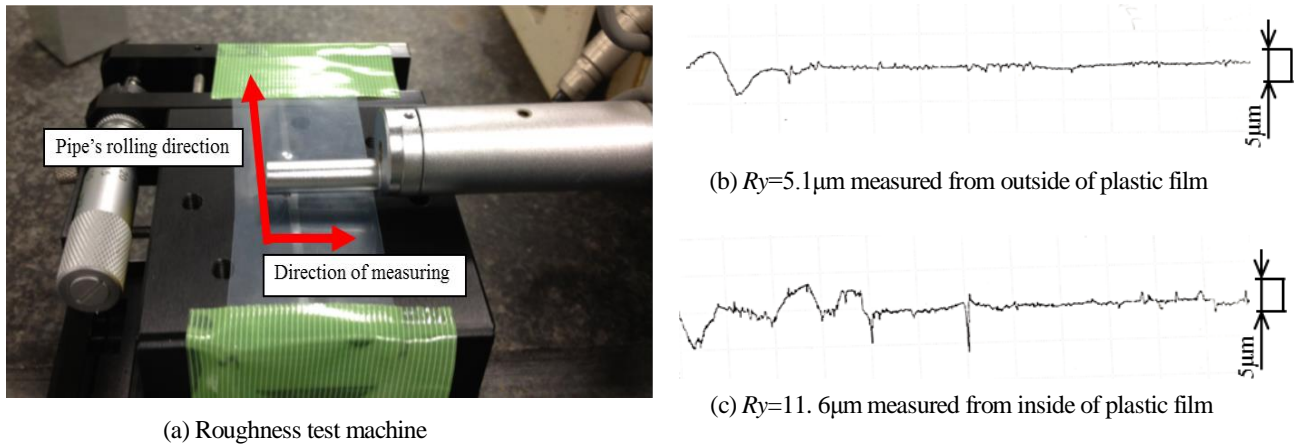
Fig. 4 (a) Surface roughness of plastic film B measured along the transverse direction of rolling. (b), (c) Maximum height: R_y is measured based on JIS (JIS B 0601). The results show that R_y observed from inside surface is about two times larger than the one observed from outside surface.
