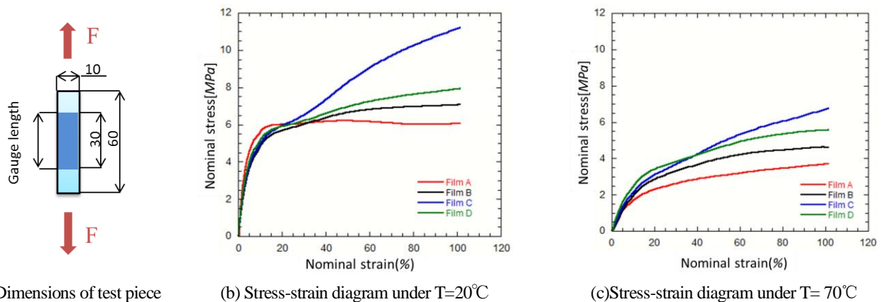
Fig. 6 Stress-Strain Diagram for different plastic film A, B, C, D. (a) Dimensions of test piece. (b) Tensile test results under T=20^{\circ}\text{C} . (c) Tensile test results under T=70^{\circ}\text{C} .
