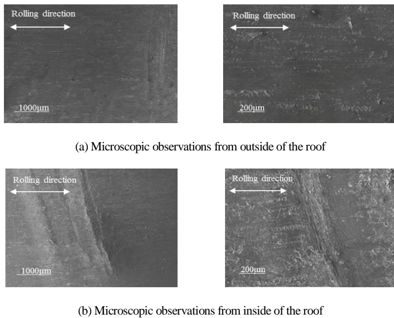
Fig. 3 Damaged plastic film observed from both outside and inside by SEM. (a) Microscopic observations from outside. (b) Microscopic observations from inside. The number of line scars observed from inside surface is more than the number of line scars observed from outside surface.
