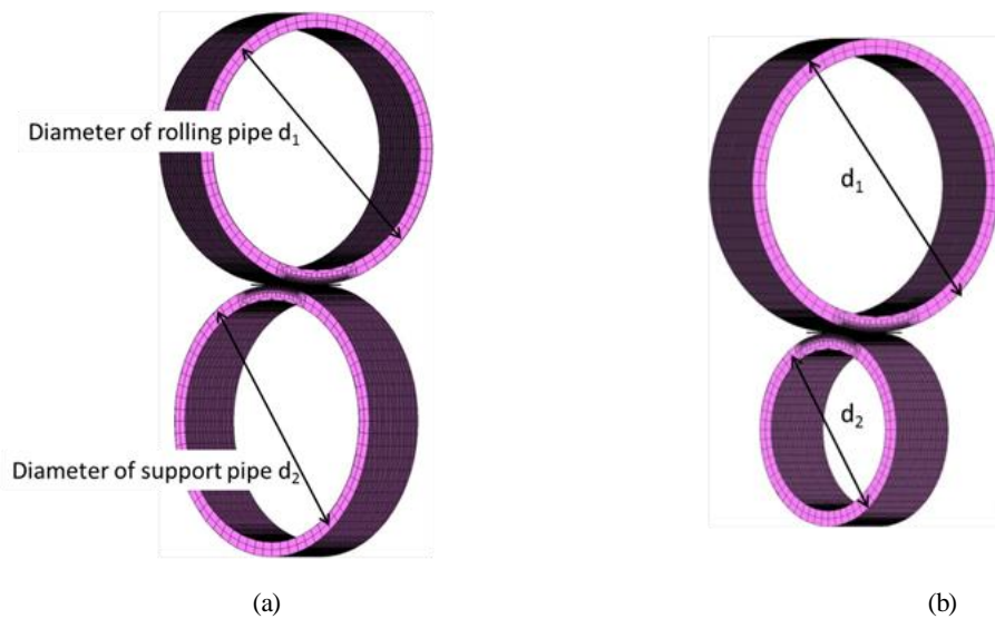
Fig. 12 3D contact models for the different dimension of support pipe. (a) Both support and rolling pipes have the same dimensions d_1=d_2=38\text{mm} . (b) Rolling pipe has the dimension d_1=38\text{mm} , and support pipe has the dimension d_2=25\text{mm} .
