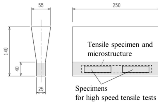
Fig. 5. Schematic view of JIS Type II Y-shaped block (in mm) and specimen positions.
