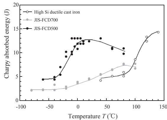
Fig. 2. Results of Charpy impact test of JIS–FCD500, JIS– FCD700 [6,7] and high–Si ductile cast iron, the tensile strength of which is nearly the same as that of JIS–FCD500.
