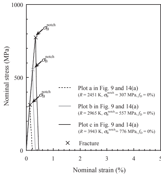
Fig. 16. Stress–strain curves of plot a (a), plot b (b) and plot c (c) in Figs. 9 and 14.
