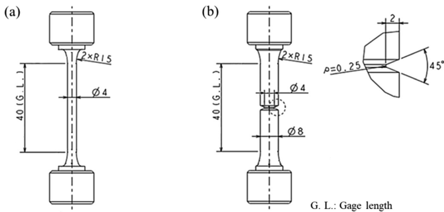
Fig. 7. Configuration of high-speed tensile test specimen (in mm): smooth specimen (a) and notched round bar specimen (b).
