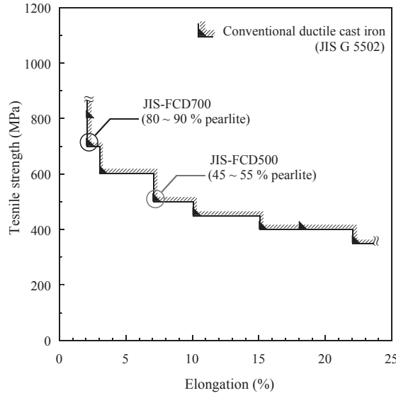
Fig. 1. Tensile strength and elongation of ferrite–pearlite ductile cast iron [1].
