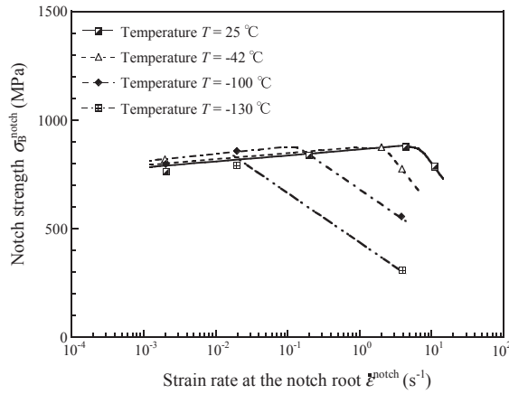
Fig. 13. Notch strength \sigma_B^{\text{notch}} of high-Si ductile cast iron in terms of strain rate \dot{\epsilon}^{\text{notch}} in temperature range of -130 – 25 °C.
