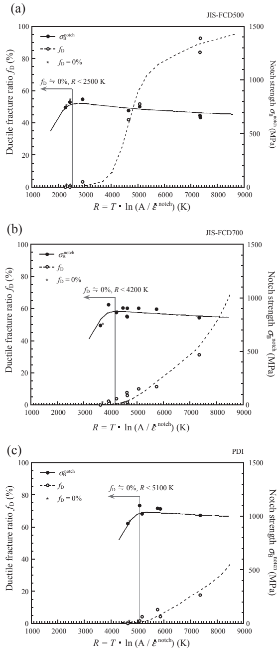
Fig. 17. Ductile fracture ratio on the notched specimen in comparison with \sigma_B^{\text{notch}} for JIS-FCD500 (a), JIS-FCD700 (b), and PDI (c).
