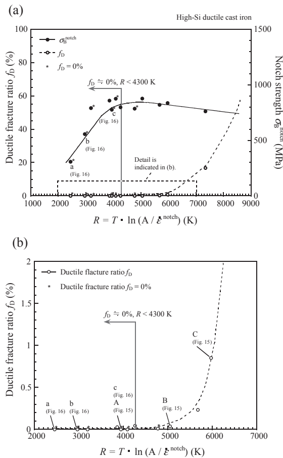
Fig. 14. Ductile fracture ratio on the notched specimen in comparison with \sigma_B^{\text{notch}} for high Si ductile cast iron: all data (a), enlarged view in the dotted line (b).
