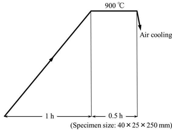
Fig. 4. Normalizing condition for PDI.
