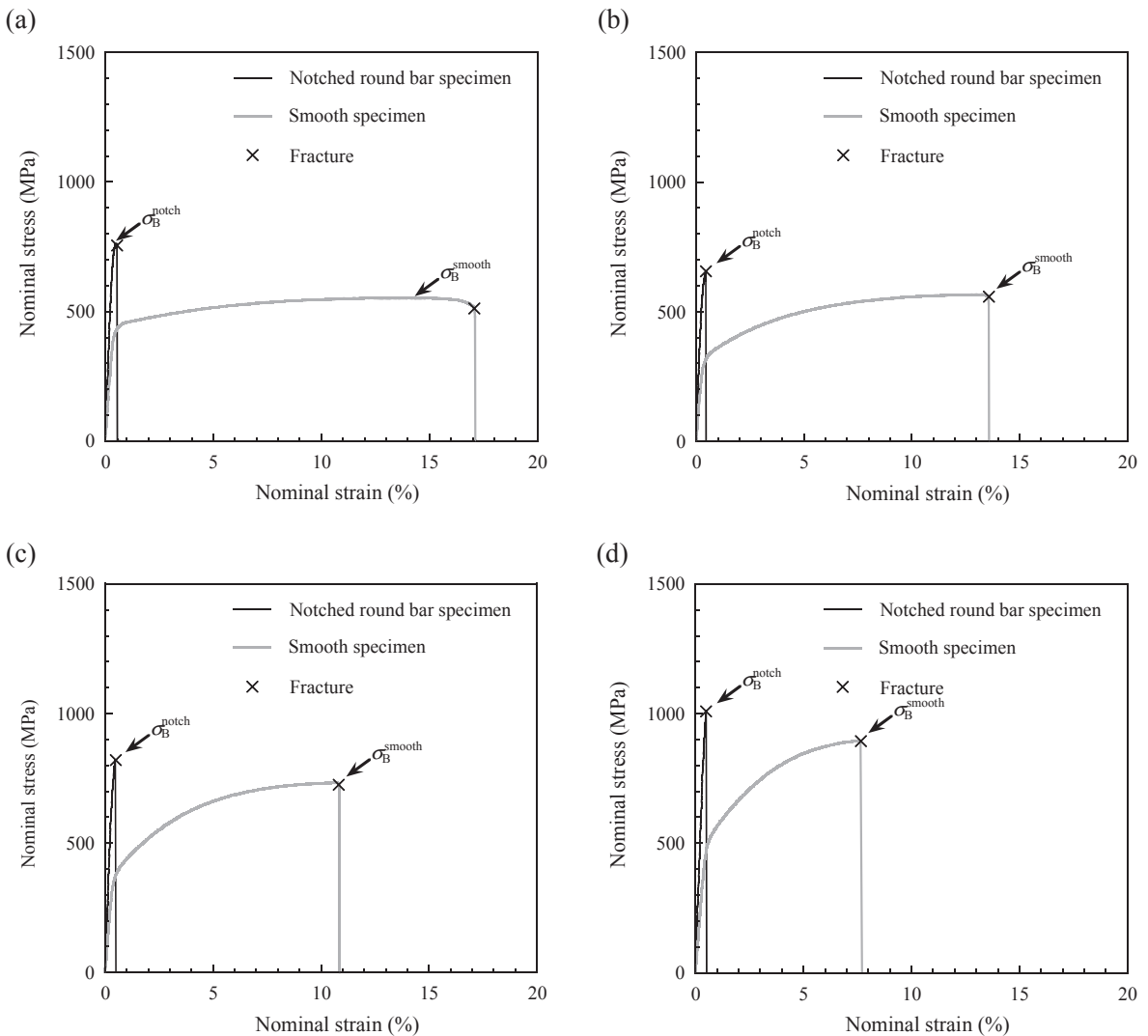
Fig. 12. Stress-strain curves of notched and smooth round bar specimens under static tensile test at temperature T = 25\text{ }^\circ\text{C} : high-Si ductile cast iron (a), JIS-FCD500 (b), JIS-FCD700 (c), and PDI (d).
