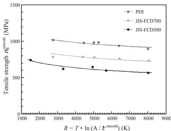
Fig. 10. Tensile strength \sigma_B^{\text{smooth}} of JIS–FCD500, JIS–FCD700, and PDI in terms of parameter R .
