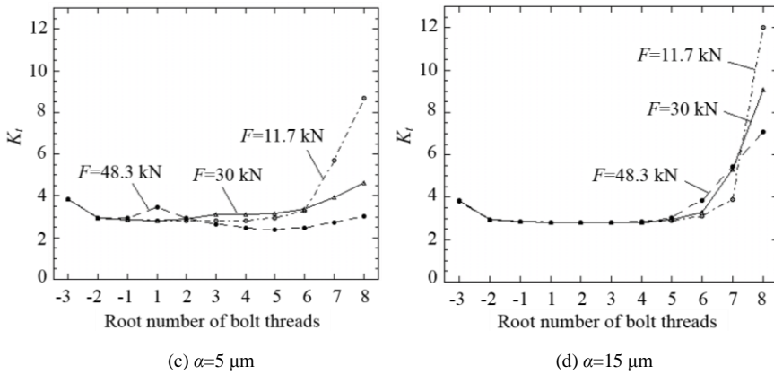
Figure 7 Stress concentration factor K_t at the root of bolt thread
